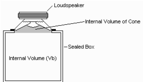
Figure 3 - Setup for Measuring V_{as}
