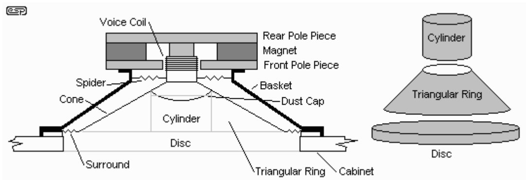
Figure 4 - Determining the Volume of the Cone
