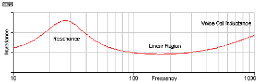
Figure 1 - Loudspeaker Impedance Curve
