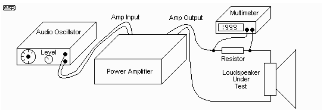
Figure 2 - Measuring the Main Speaker Parameters
