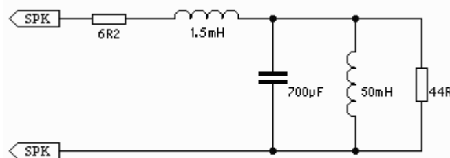
Figure 5 - Dummy Test Loudspeaker
