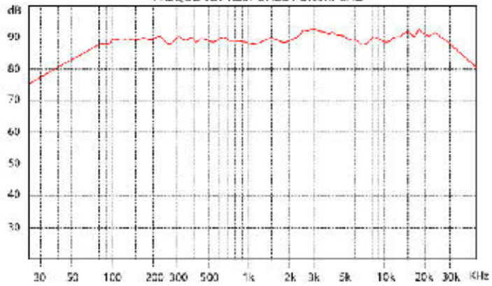
EJ JORDAN DESIGNS, U.K. FREQUENCY RESPONSE FOR JXR6HD
